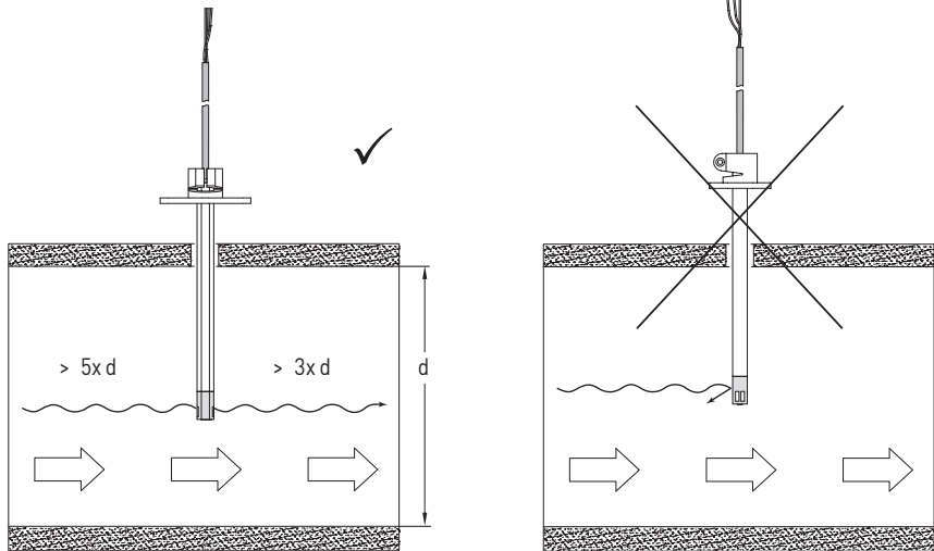
Mounting diagram
