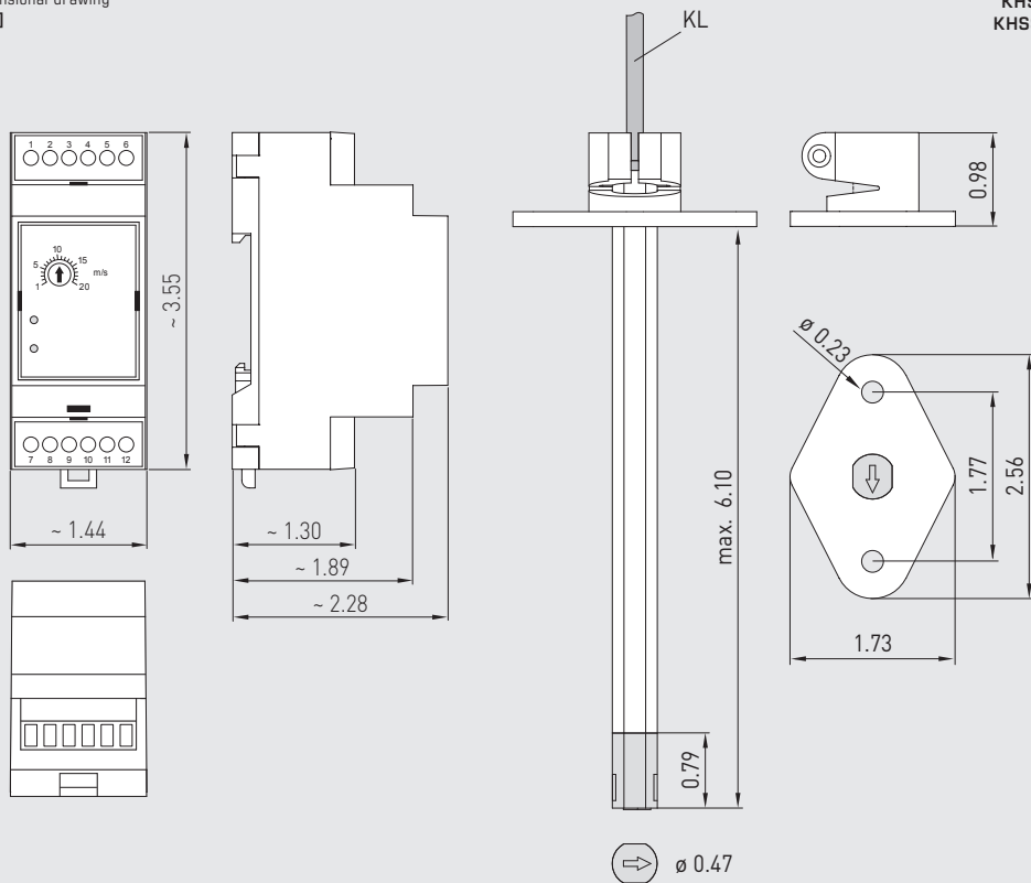
Dimensional drawing [inch]
