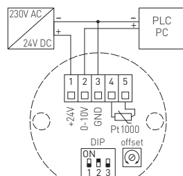
Schéma de raccordement RGTM 1-U
