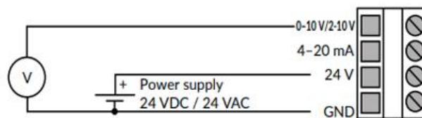
Figure 2a - Wiring diagram voltage output
