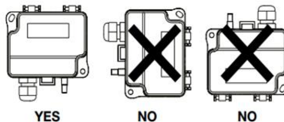
Figure 1a - Mounting orientation
