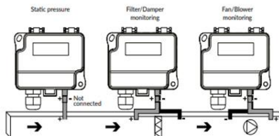
Figure 1b - Application connections
