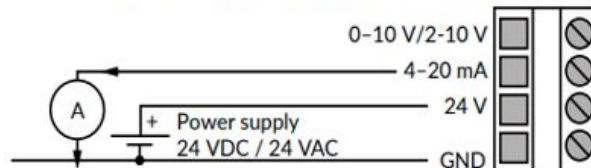
Figure 2b - Wiring diagram current output
